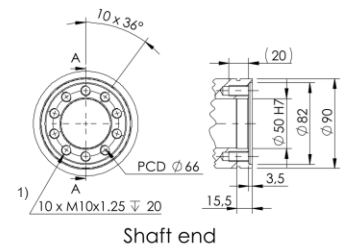
Shaft end
